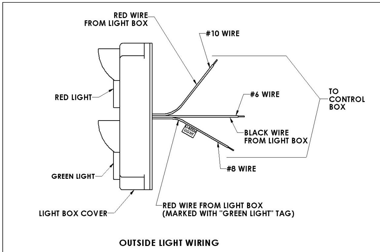
FIGURE G—OUTSIDE LIGHT BOX WIRING
