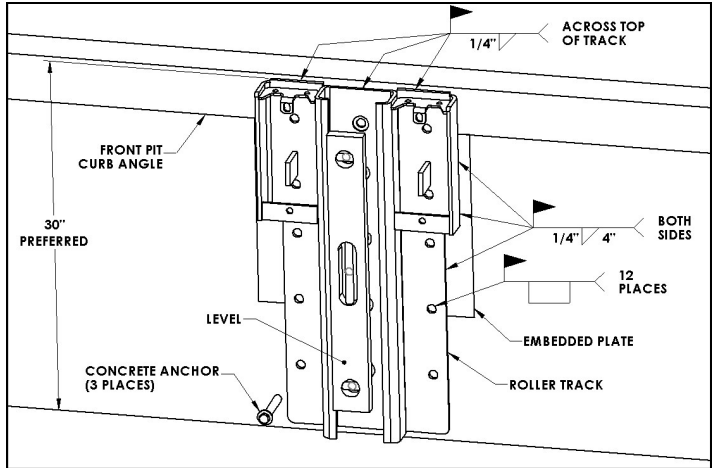
FIGURE C—WELDING ROLLER TRACK (WITH EMBEDDED PLATE)
