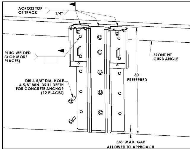
FIGURE D—WELDING ROLLER TRACK
