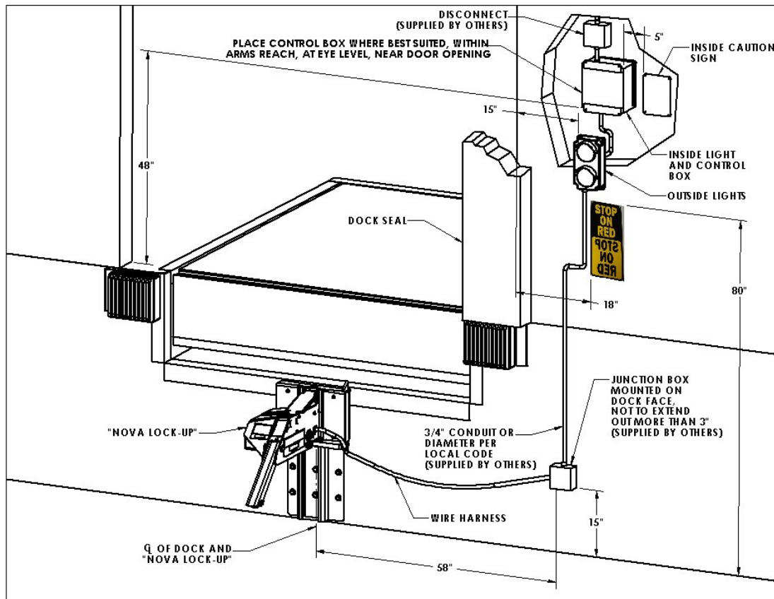
FIGURE H—SUGGESTED COMPONENT LOCATION
