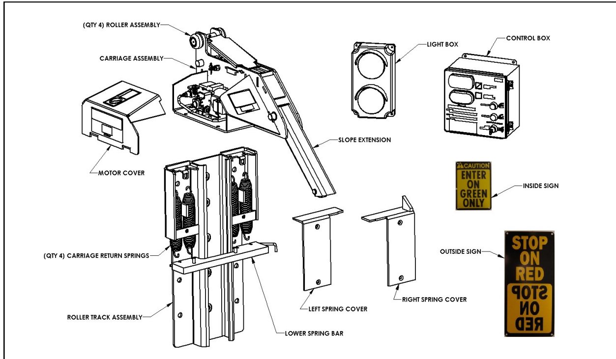
FIGURE A — PARTS IDENTIFICATION
