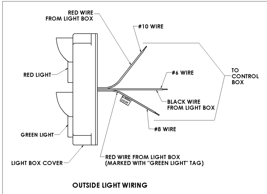
FIGURE G—OUTSIDE LIGHT WIRING
