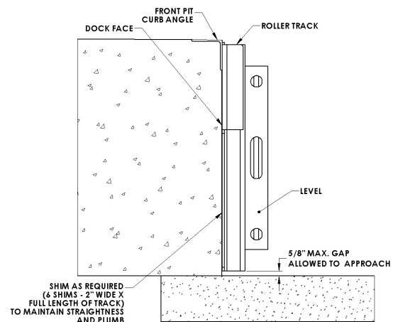
FIGURE D—WELDING ROLLER TRACK SIDE VIEW
