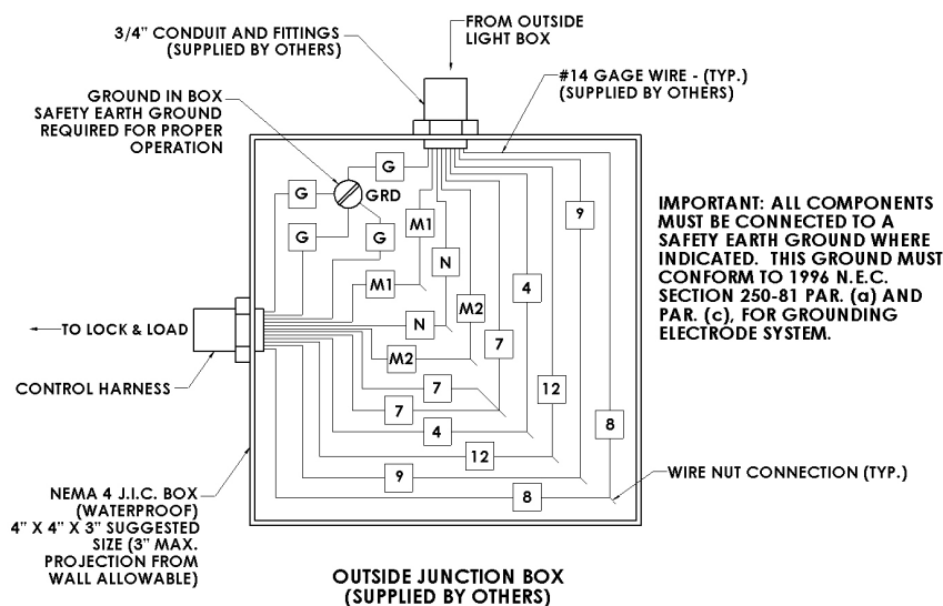
FIGURE F—OUTSIDE JUNCTION BOX
